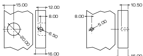
F301 with 15 mm tie-rod
